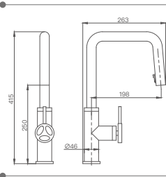
AQL043 Kitchen Faucet Material: Brass Surface Treatment: Chrome
