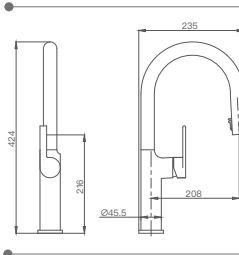
AQL041 Kitchen Faucet Material: Brass Surface Treatment: Chrome
