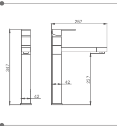
AQ8145NGBN Kitchen Faucet Material: SS304 Surface Treatment: Brush
