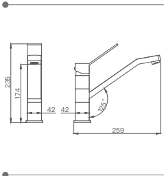
AQ814NGBN Kitchen Faucet Material: SS304 Surface Treatment: Brush
